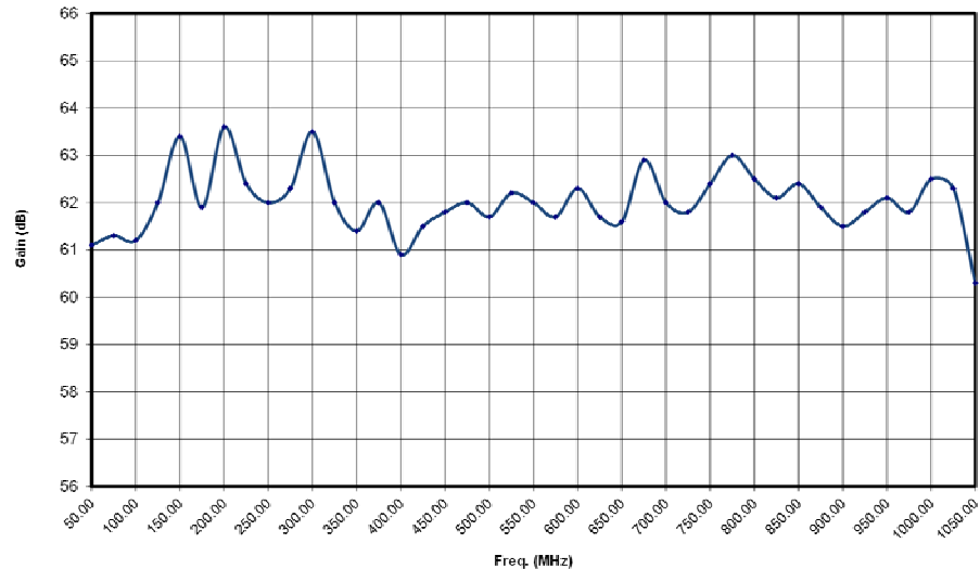
500W1000B Typical Gain flatness @ -20 dBm input
