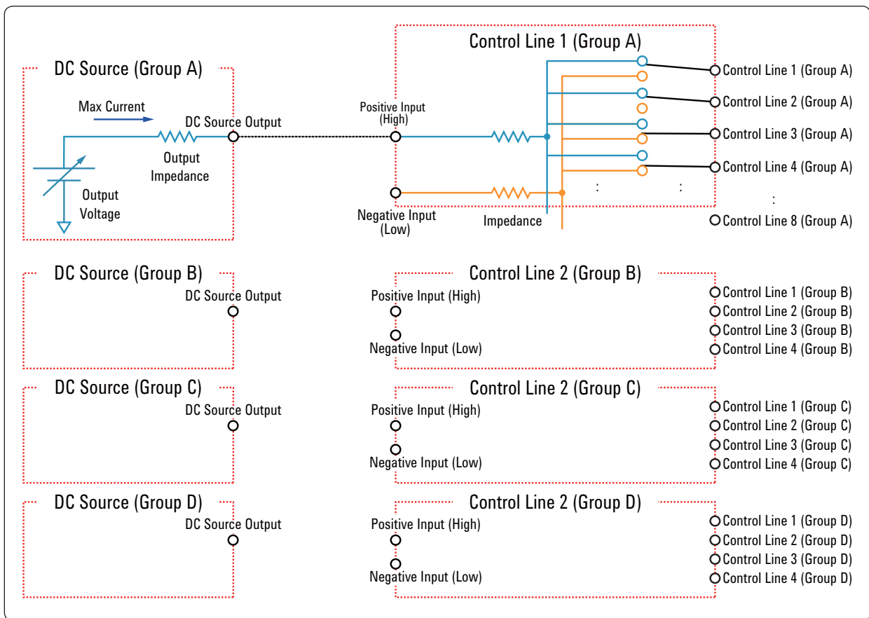
Figure 3-6. DC control line (E5092A-020)
