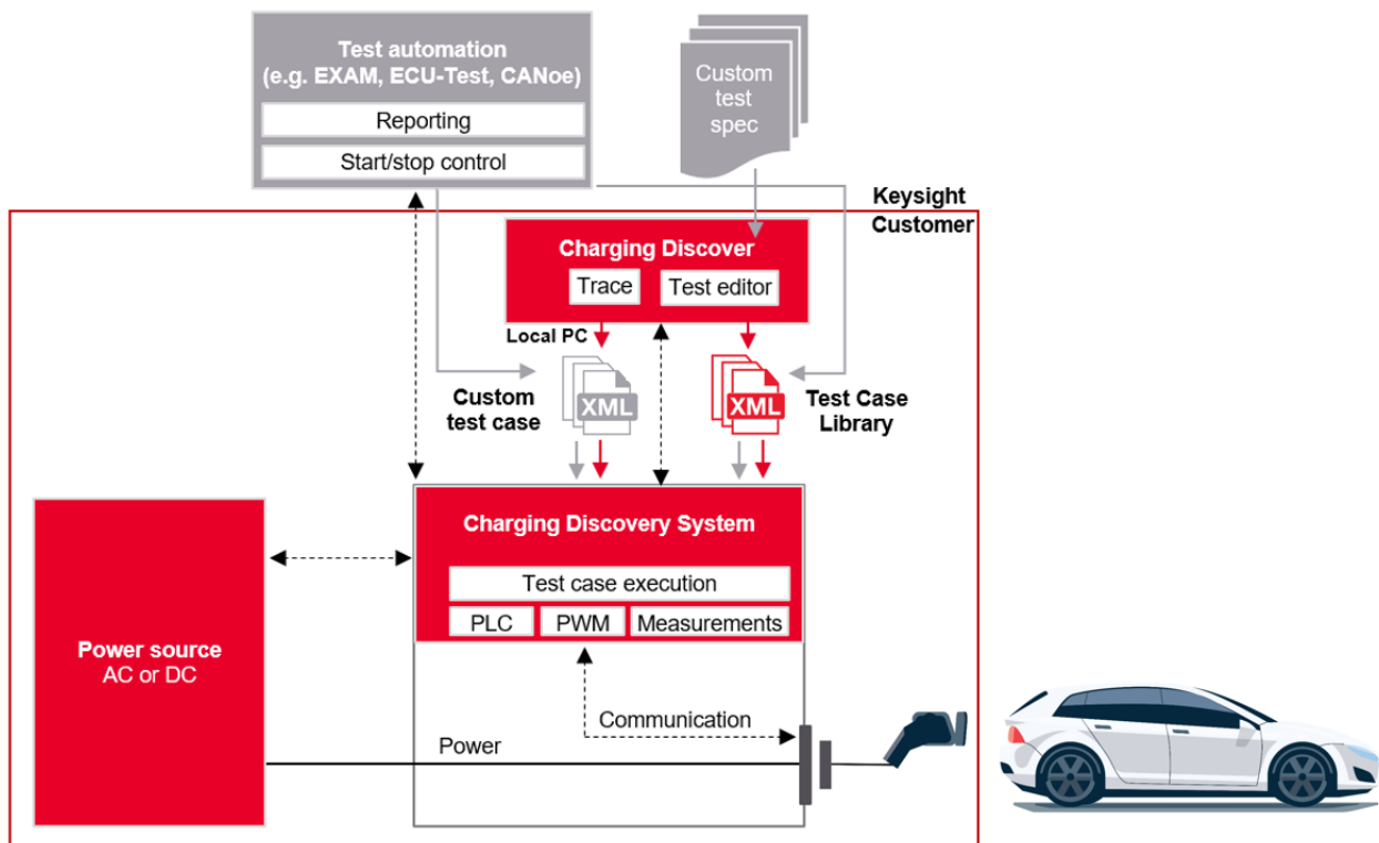
Figure 6. Interface topology of CDS with Expert mode.
