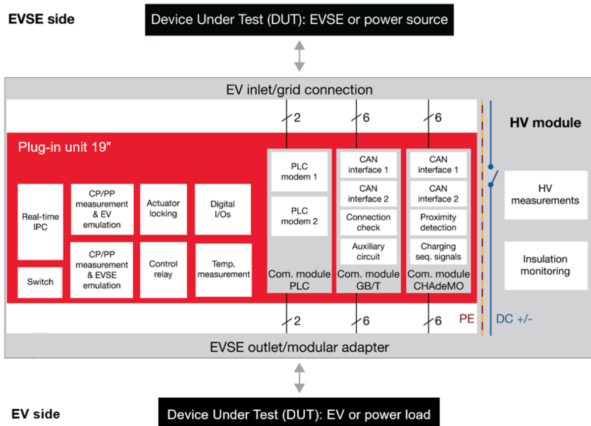
Figure 2. Block diagram of CDS architecture.
