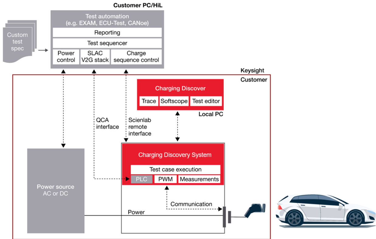
Figure 7. Interface topology of CDS with Developer mode.
