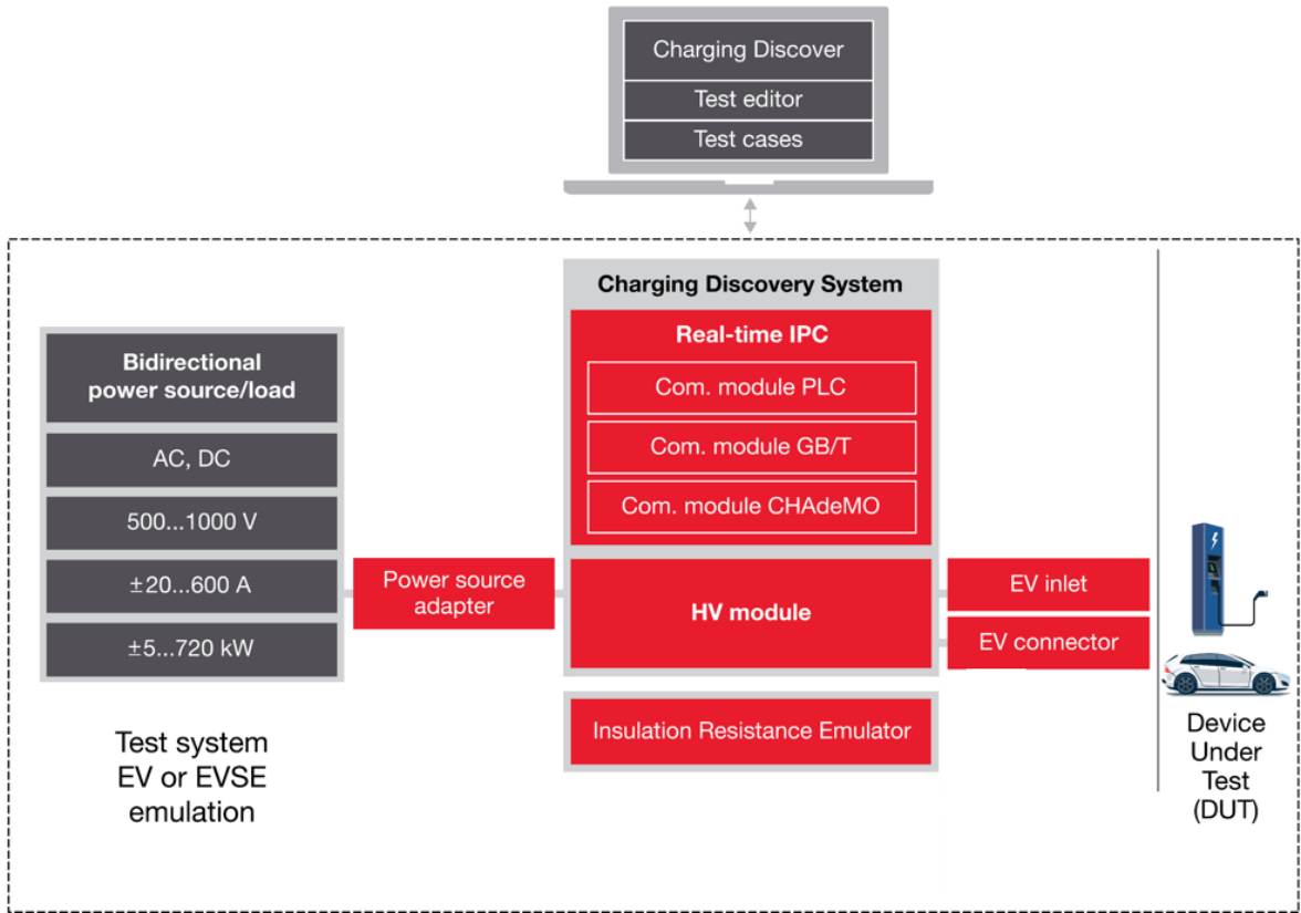
Figure 1. Modularity of the Scienlab Charging Discovery System – Portable Series.
