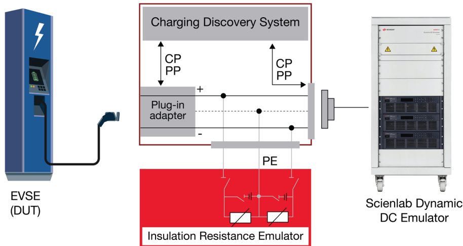
Figure 3. System topology including Scienlab Isolation Resistance Emulator.
