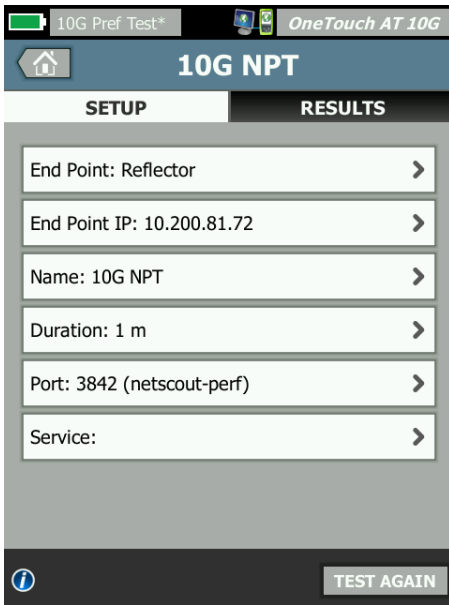
Figure 16: 10G NPT tests up to 10G against reflector, peer or OptiView XG over a user defined UDP port.
