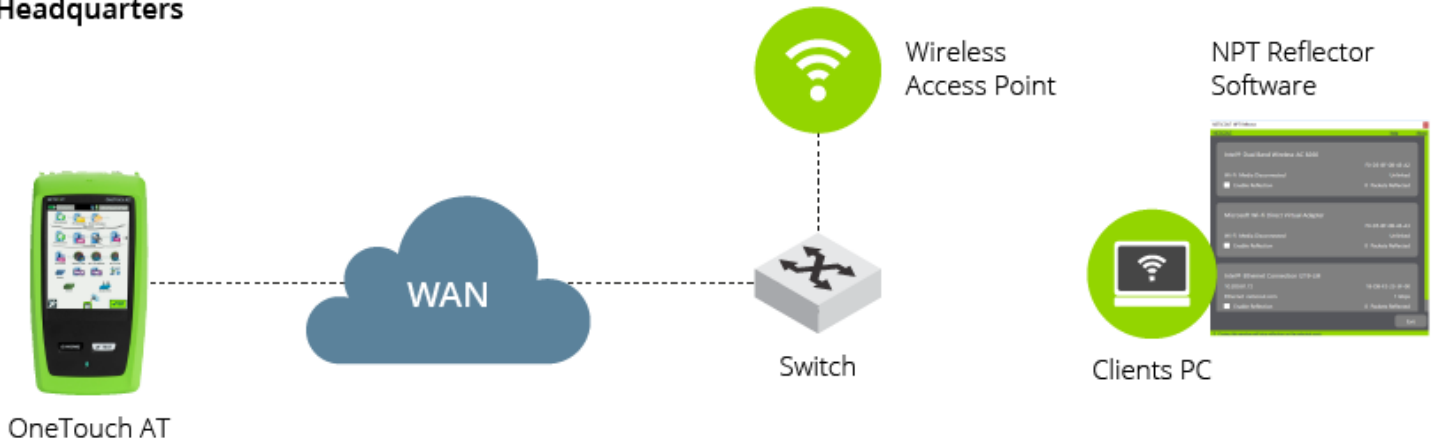
Figure 14: The NPT Reflector can be downloaded directly from OneTouch G2 or 10G to a Windows PC at a remote site to validate network performance.
