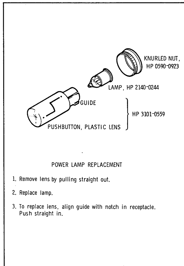
Figure 3-1. Lamp Replacement
