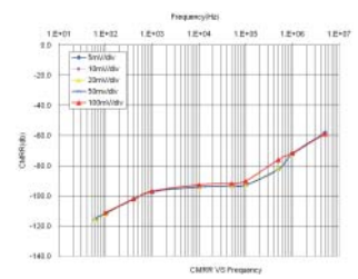
Model 701250 Voltage Input Module
