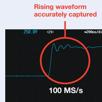
Example: Same inverter output waveform measured at 10 MS/s and 100 MS/s
