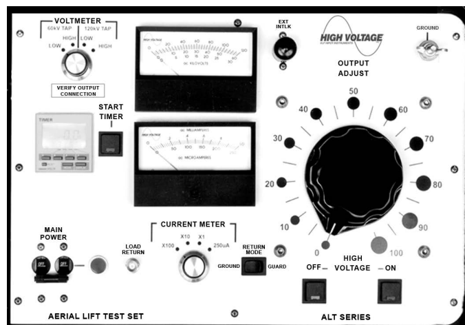
Control Layout
