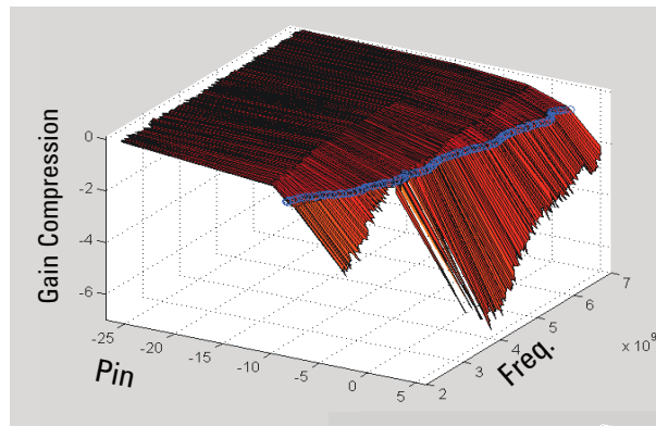
Measured background data in SMART Sweep with Safe Mode Off (above) and On (below)—more iterations are used as the gain becomes closer to the 1 dB compression point with Safe Mode On, which minimizes excess drive power.
