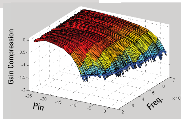
Measured background data in SMART Sweep with Safe Mode Off (above) and On (below)—more iterations are used as the gain becomes closer to the 1 dB compression point with Safe Mode On, which minimizes excess drive power.
