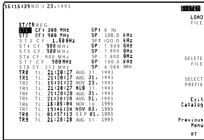
Figure 3-17. Catalog Analyzer Internal Memory
