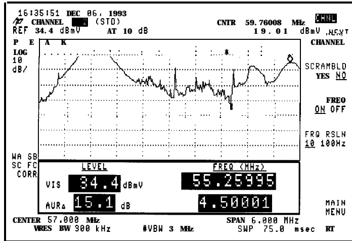
Figure 2-8. 10 Hz Resolution
