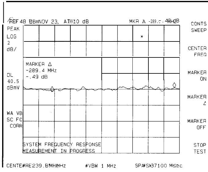
Figure 2-39. System Frequency Response Measurement
