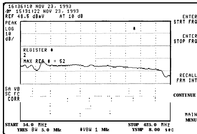
Figure 5-9. Trace B, Recalled
