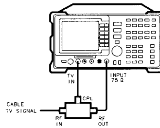
Figure 3-4. Connections for HP 8591 C analyzer with Option 107 (RF Measurements)
