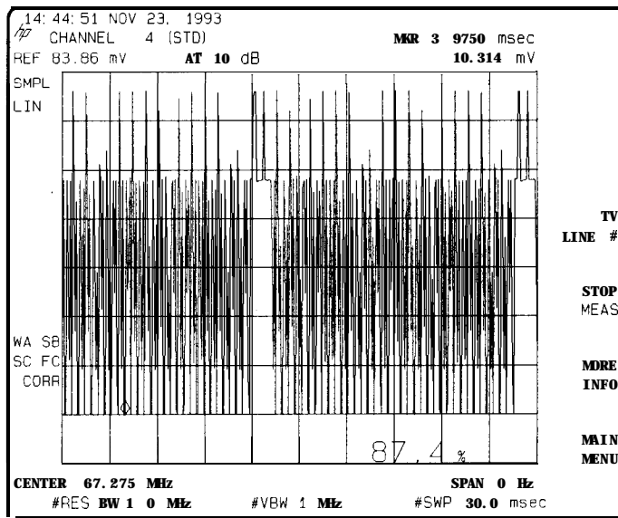
Figure 8-9. Measuring the Depth of Modulation
