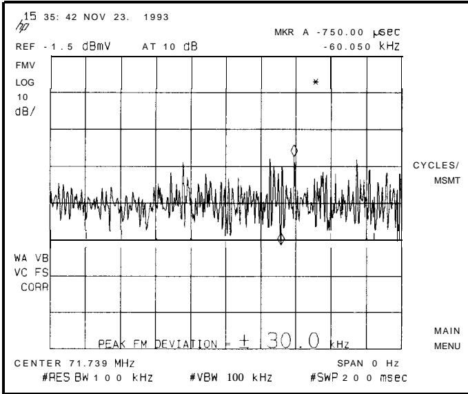
Figure 2-29. FM Deviation
