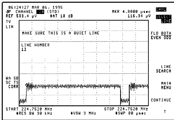
Figure 2-11. Example of a Quiet line
