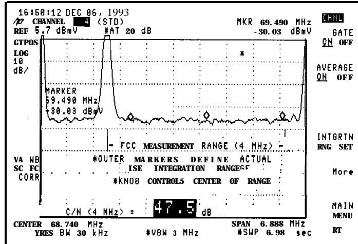
Figure 8-3. Carrier-to-Noise Measurement
