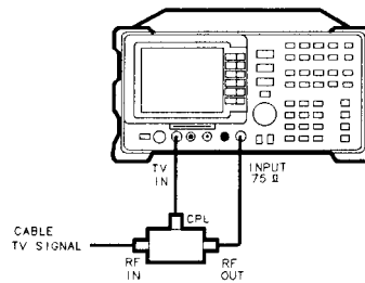
Figure 2-5. Connections for HP 8591C analyzer with Option 107
