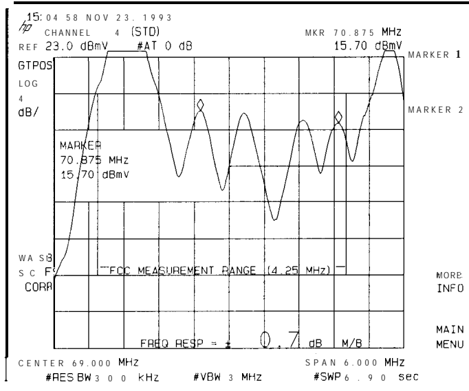
Figure g-17. Multi-Burst Response
