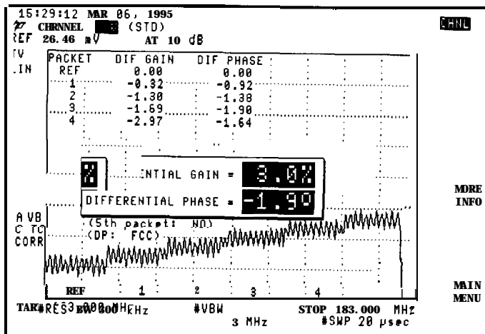
Figure g-15. Differential Gain/Differential Phase
