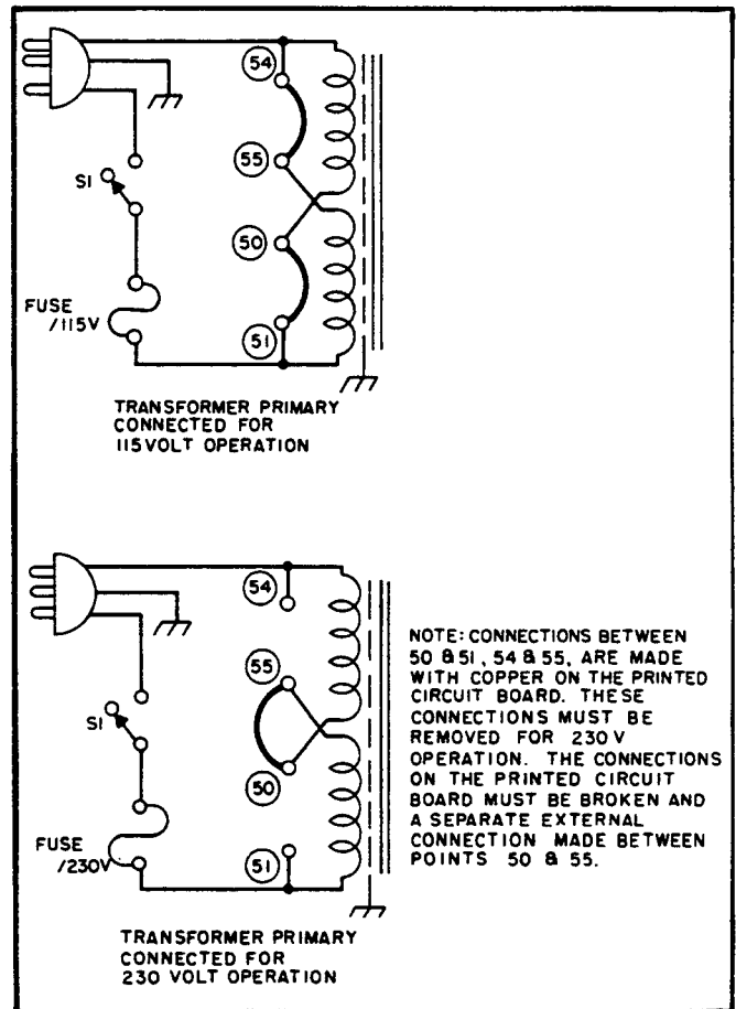
Figure 2-1. Primary Connections
