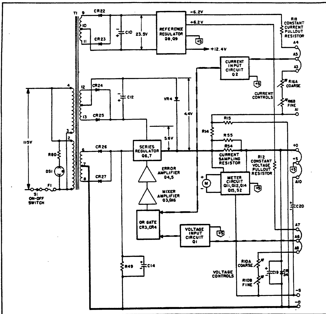
Figure 4-2. Simplified Schematic
