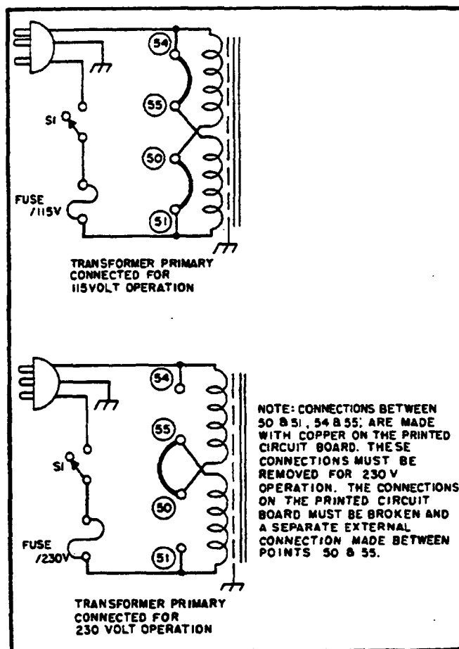
Figure 2-1. Primary Connections
