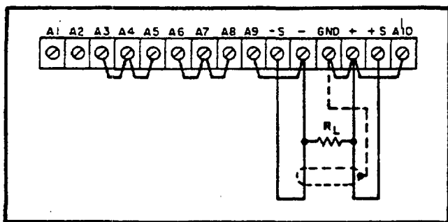
Figure 3-7. Remote Sensing
