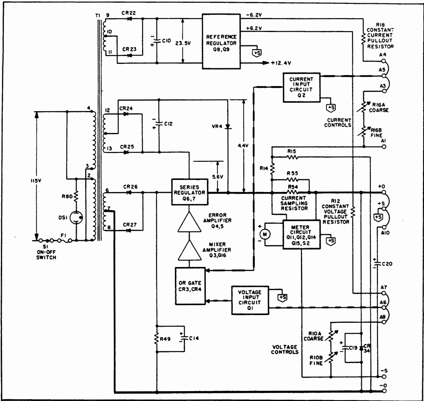
Figure 4-2. Simplified Schematic
