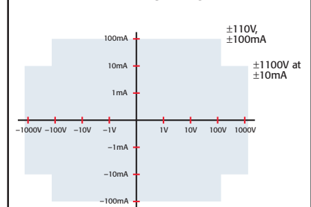
Model 237 Source Capability
