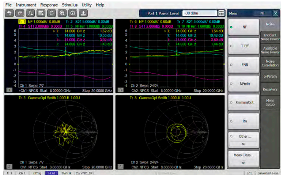
Unmatched device noise parameter measurements with ECal as impedance tuner vs with Maury LXI tuner as impedance tuner.
