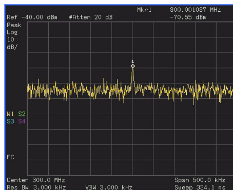
Figure 3-10 A signal closer to the noise level
