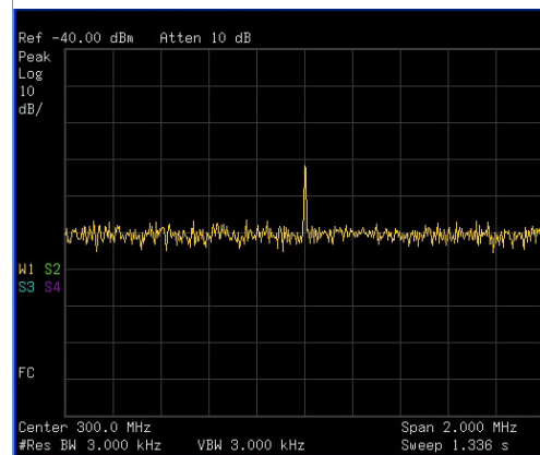
Figure 3-12 Decreasing Resolution Bandwidth
