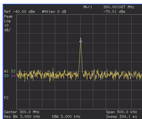
Figure 3-11 Measuring a low-level signal using 0 dB Attenuation
