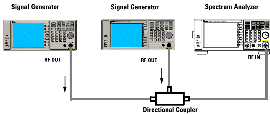
Figure 3-4 Setup for obtaining two signals
