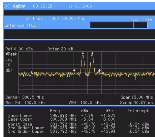
Figure 4-7 TOI Measurement
