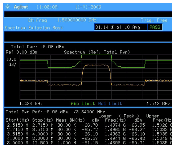
Figure 4-8 Spectrum Emission Mask
