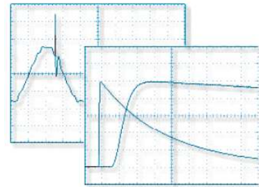
Combination wave detail (front) and impulse on AC power frequency (rear)
