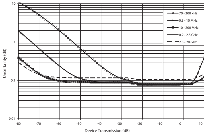
Transmission Magnitude Uncertainty (1 of 2) MS4647A with SOLT Calibration using 3654D Cal Kit
