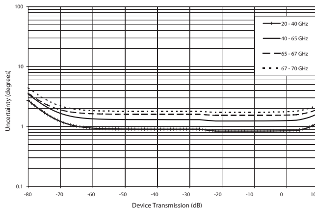
Transmission Phase Uncertainty (2 of 2) MS4647A with SOLT Calibration using 3654D Cal Kit
