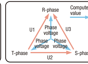
Figure 2 Delta-star conversion
