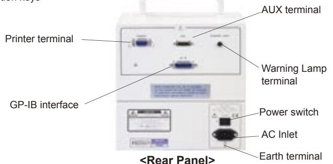
<Rear Panel>
