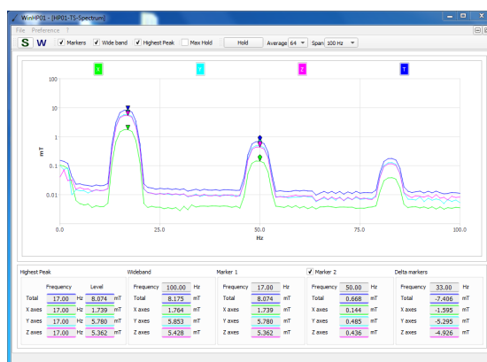
Figure 7: FFT analysis with display of amplitude spectrum
