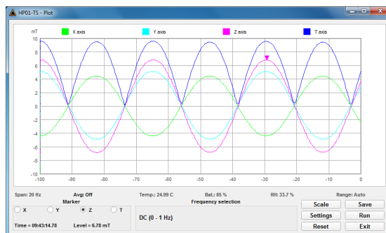
Figure 6: Time response display of a sine wave signal in the sub-Hertz range in DC-1Hz operating mode
