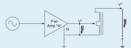
Single Phase Transformer Coupled Power Source
