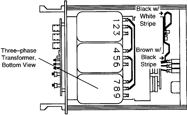
Illustration 3-33 380 Vac Transformer Wiring
