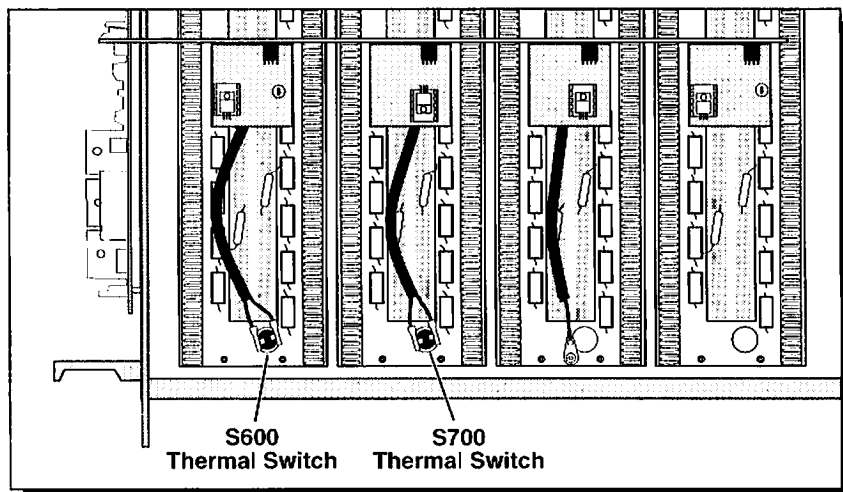
Illustration 6-14 Thermal Switch Location
