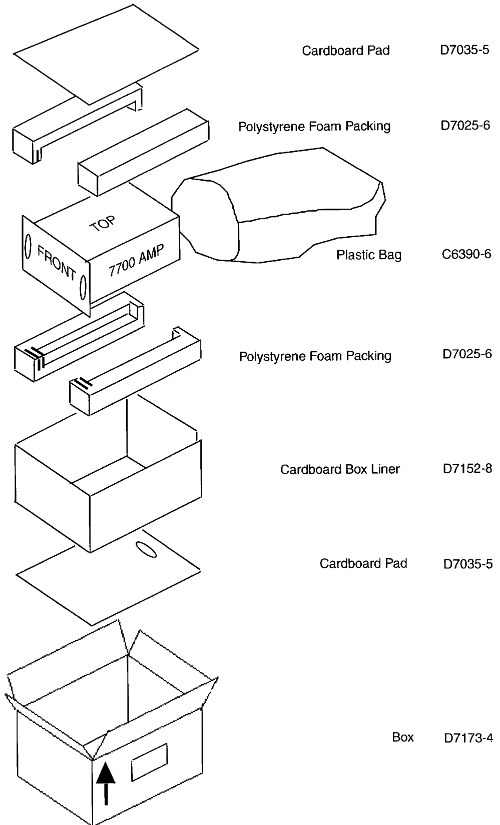
Illustration 5-7 Packing Materials for Shipping 7700 Amplifiers
