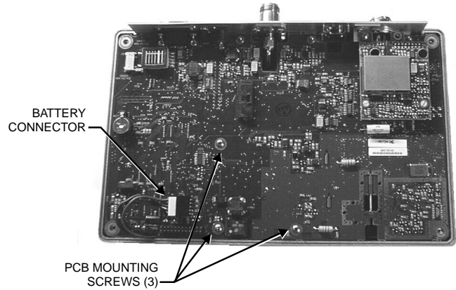
Figure 16. Control PCB
