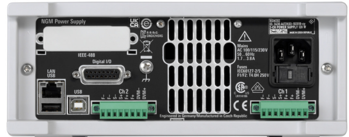
R&S®NGM202, rear view
