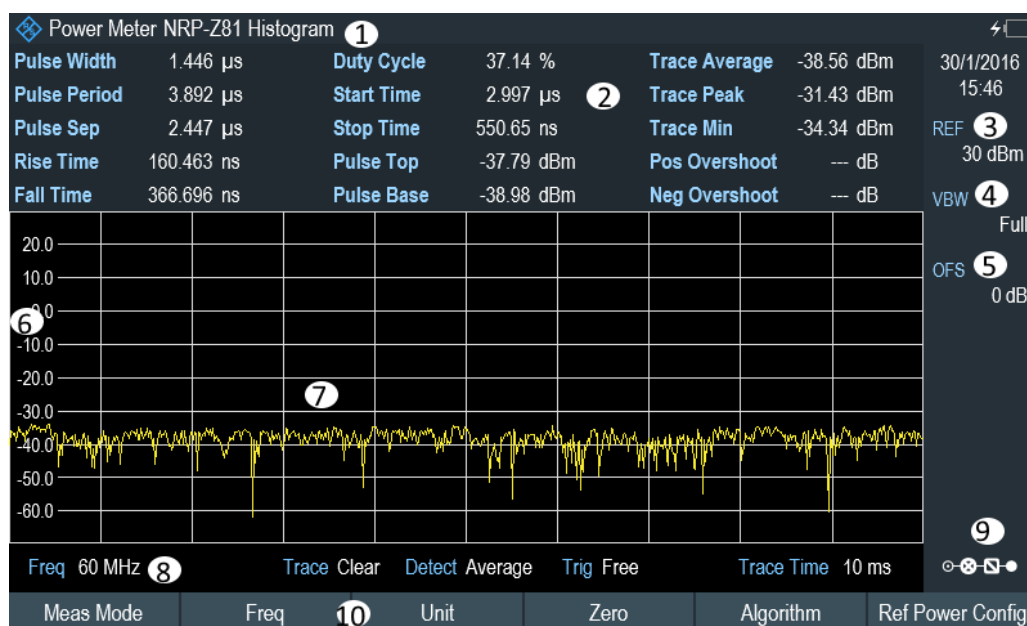
Figure 9-1: Power vs time display
