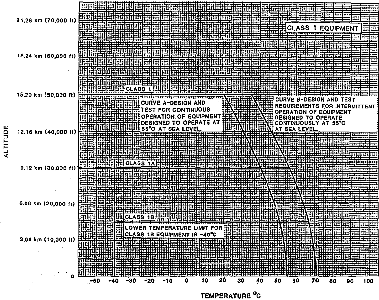
FIGURE 1. Operational guidelines for class 1 airborne electronic equipment (temperature vs altitude).
