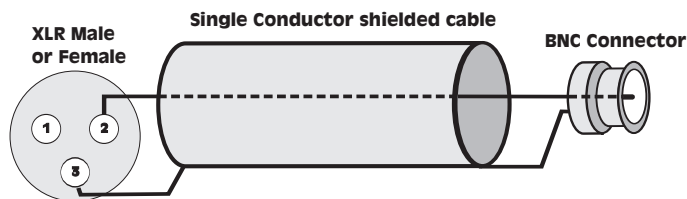
Figure 3-19. Unbalanced connections using single-conductor cable
