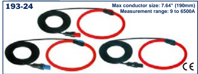
Set of three color-coded AmpFlex™ 193-24 (6500A) flexible current probes with 24" sensors Catalog #2140.11
