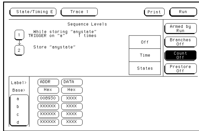
Figure 5-71. Count Pop-up Menu
