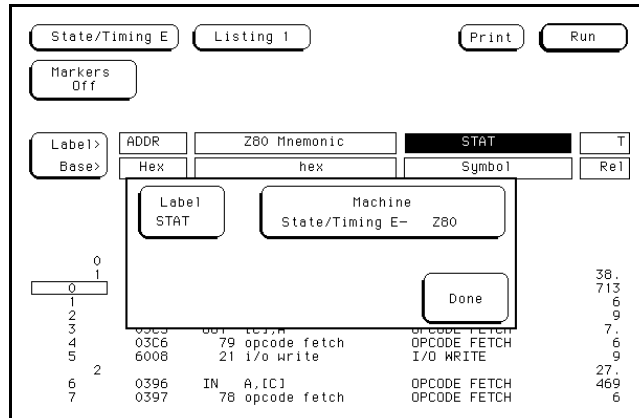
Figure 6-17. Machine and Label Pop-up Menu
