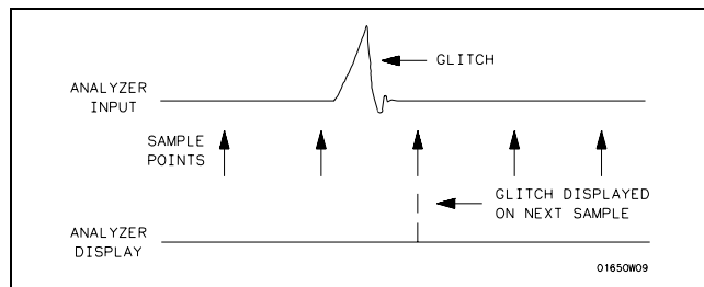
Figure 5-34. Glitch in Timing Waveform
