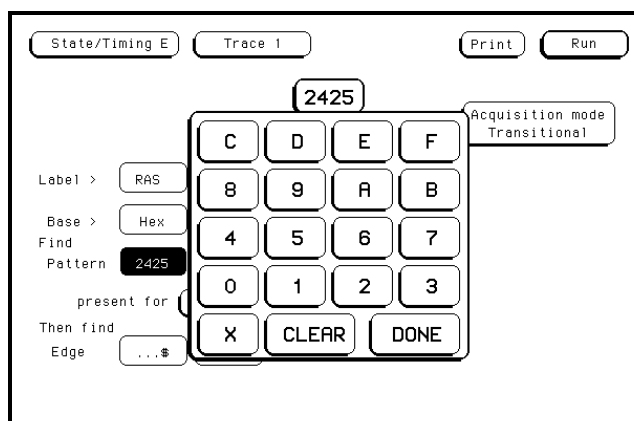
Figure 5-37. Specify Pattern Pop-up for Find
