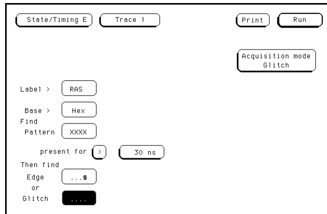
Figure 5-33. Glitch Specification Field
