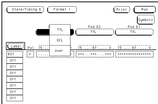
Figure 5-11. Pod Threshold Pop-up Menu
