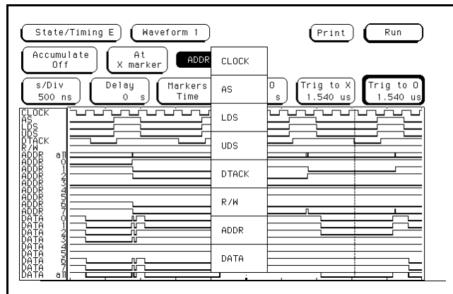
Figure 6-8. Label Option Pop-up
