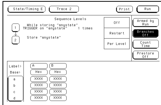
Figure 5-66. Branches Pop-up Menu
