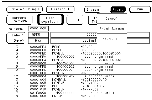
Figure 13-2. Print Option in Listing Menu
