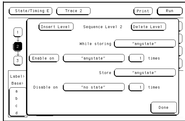
Figure 5-59. Sequence Level Pop-up with Storage
