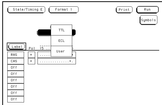
Figure 3 - 3. Pod Threshold
